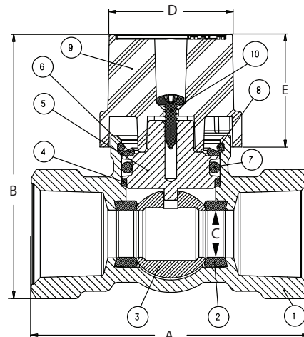
Pictured T-3001 Cut-away
